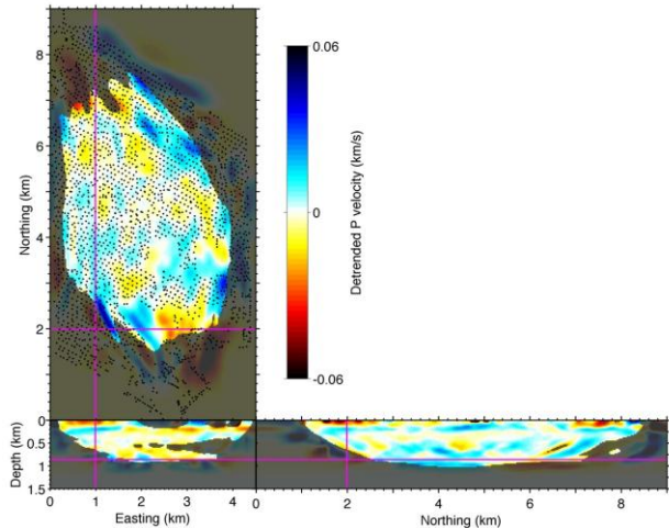
Figure 1 - Body Wave Extraction and Tomography from Ambient Noise Data
