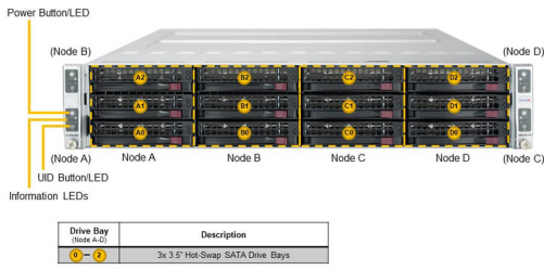
(Front View – System)
