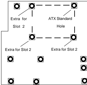
Figure 2-1. Dual Retention Module Mounting Holes
