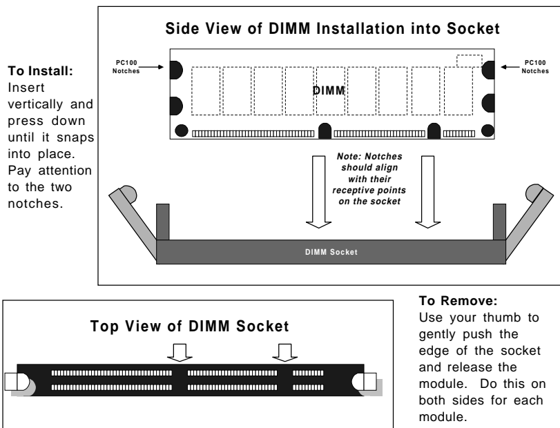
Figure 2-3. DIMM Installation
