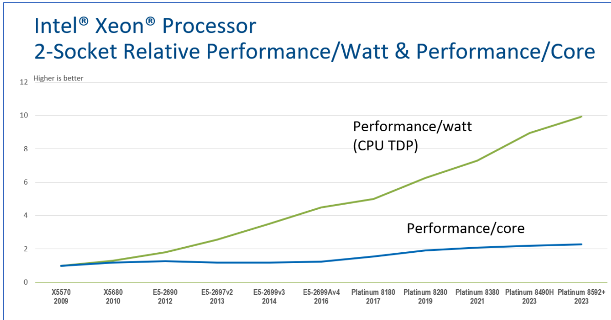
Figure 2 - Performance Per Watt Over Time Image Courtesy of Intel)
