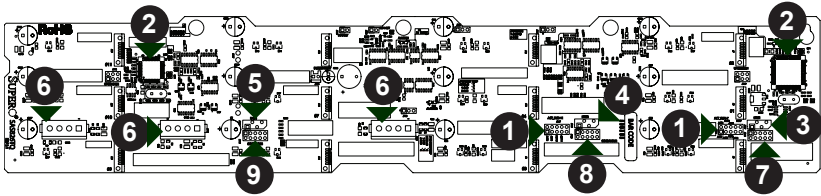
Figure 2-1: Front Connectors
