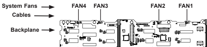
Figure 2-2. Default Configuration--Fans Connected Directly to the Backplane
