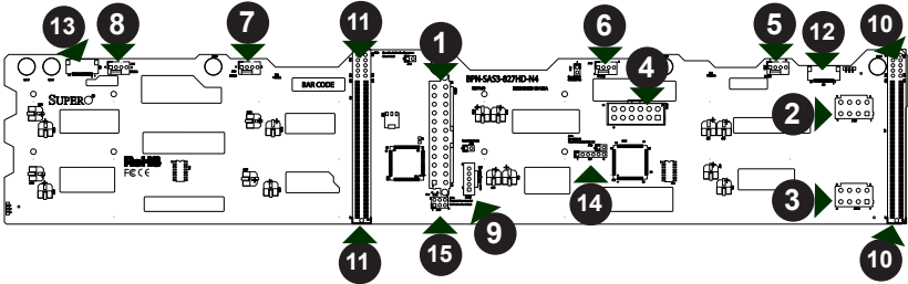
Figure 2-1. Rear Connectors
