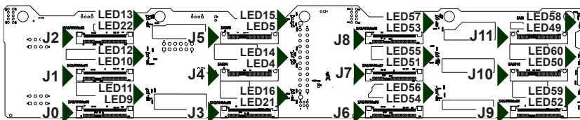
Figure 2-7. Front Connectors and LEDs
