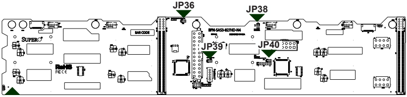
Figure 2-3. Rear Jumpers
