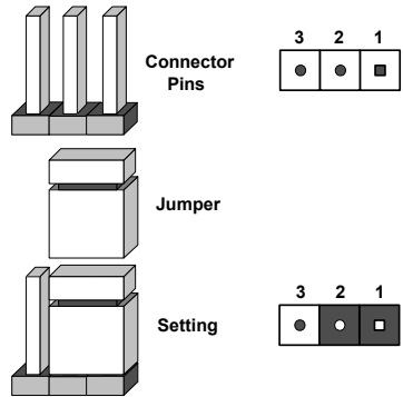
Figure 2-3. Rear Jumpers
